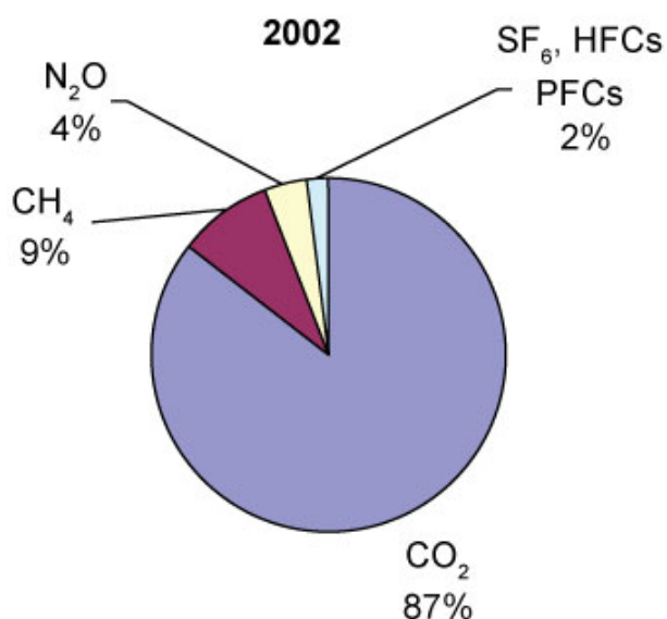
Distribution by Greenhouse Gas
