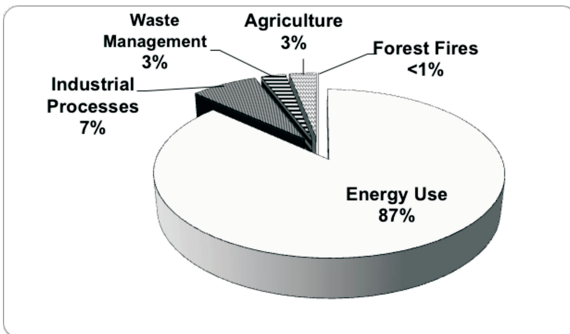
Emissions by Sector
